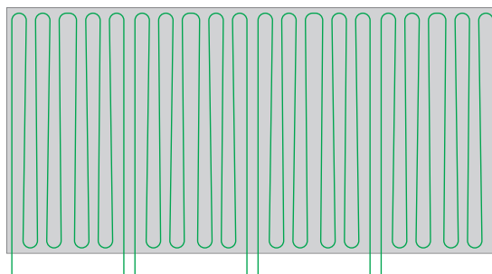
1200x600 mm 12-m Circuit/Circuito 12 m 4 elementary circuits 4 circuiti elementari
