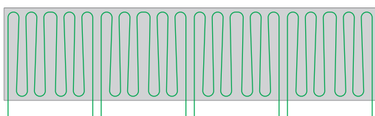
600x600 mm 6-m Circuit/Circuito 6 m 2 elementary circuits 2 circuiti elementari
