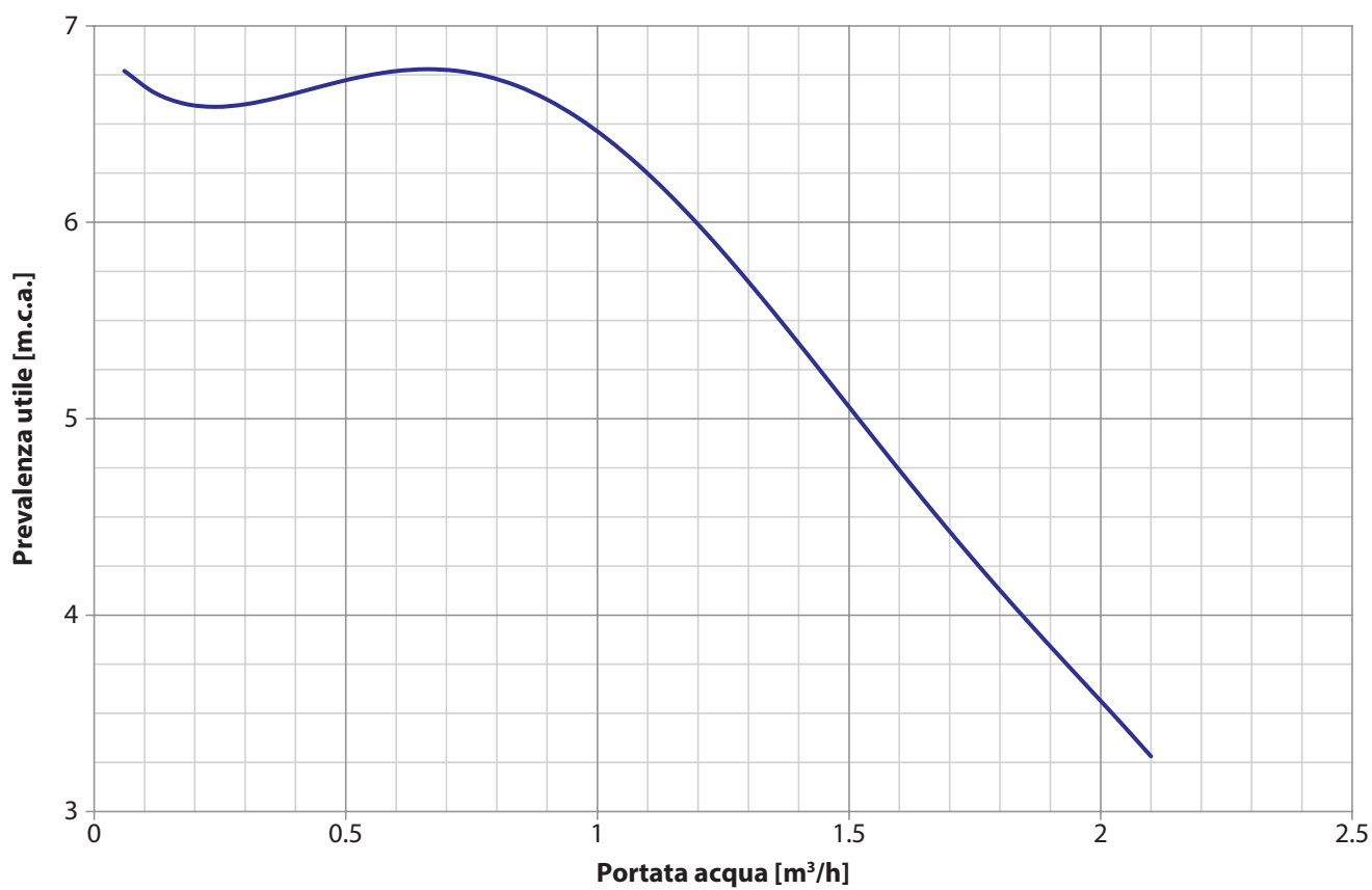
GM VJ / PF-CF DN 25
